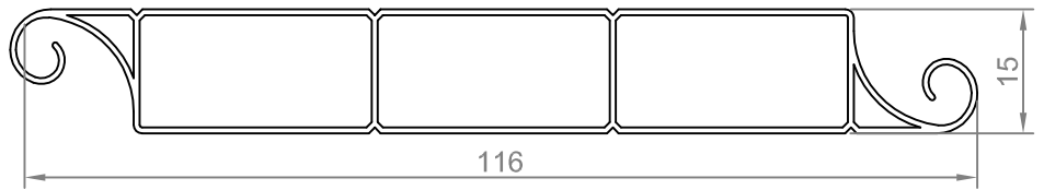
LAME PVC 116
