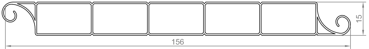
LAME PVC 156
