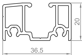
RAIL ACCES PMR ALUMINIUM
