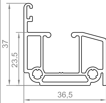
RAIL PVC
