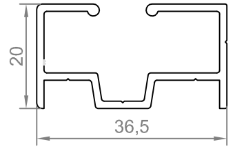
MONTANT ALUMINIUM
