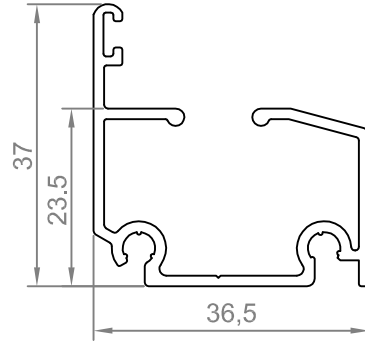
RAIL ALUMINIUM
