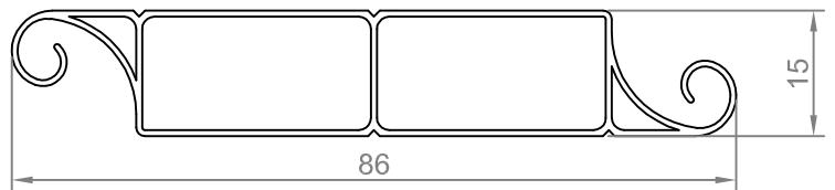
LAME PVC 86
